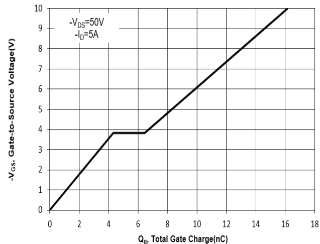
Fig. 11 Gate Charge
