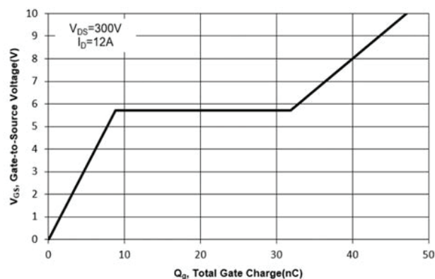
Fig. 11 Gate Charge
