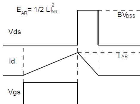
Fig.3-2 Avalanche waveform
