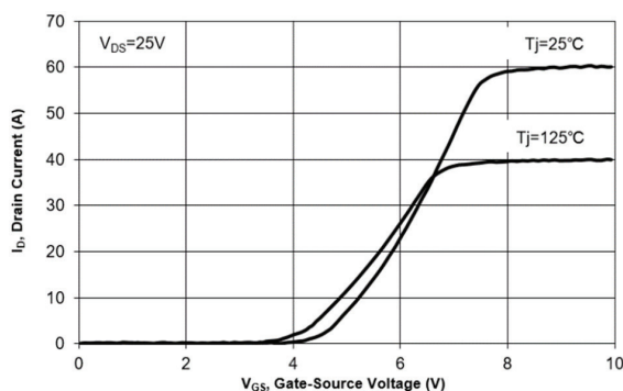
Fig. 2 Typical Transfer Characteristics
