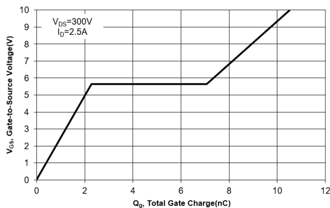
Fig. 11 Gate Charge
