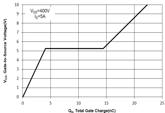
Fig. 11 Gate Charge
