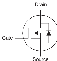
1.Gate 2.Drain 3.Source TO-220F Plastic Package
