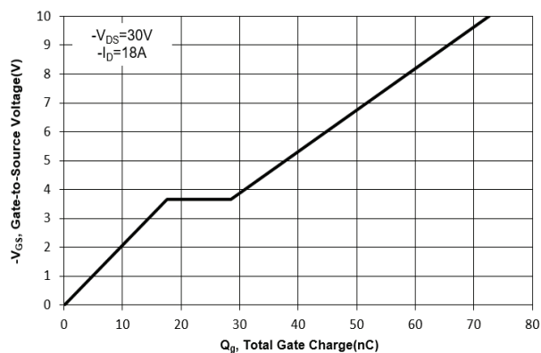
Fig. 11 Gate Charge
