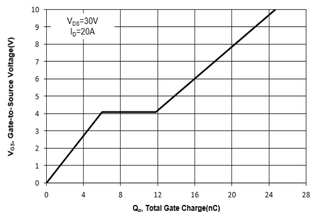
Fig. 11 Gate Charge
