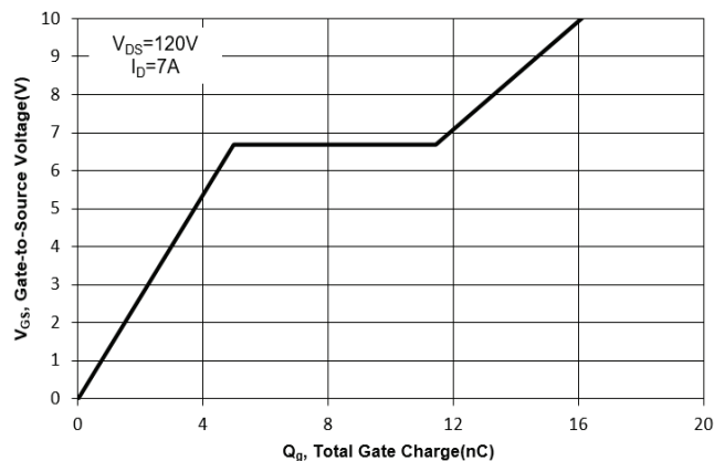
Fig. 11 Gate Charge
