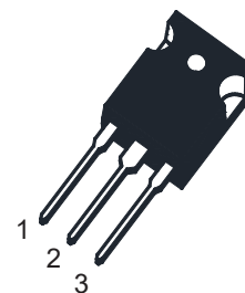
TO-247 Plastic Package 1.Gate 2.Drain 3.Source
