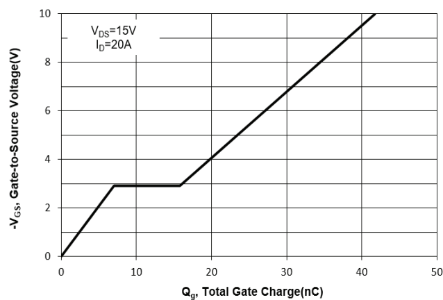
Fig. 11 Gate Charge
