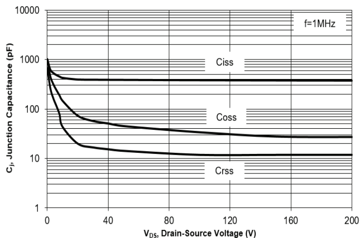
Fig. 7 Typical Junction Capacitance
