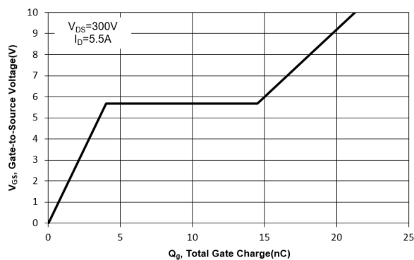
Fig. 11 Gate Charge
