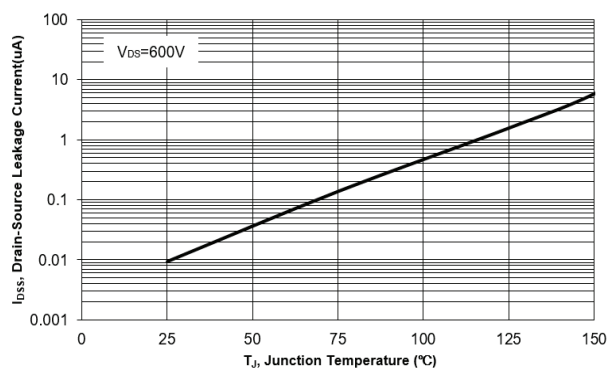
Fig. 8 Drain-Source Leakage Current vs. T_J
