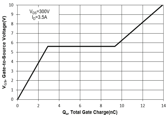
Fig. 11 Gate Charge
