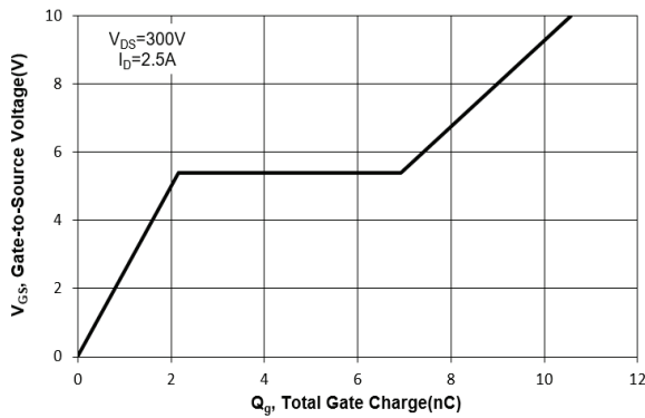
Fig. 11 Gate Charge
