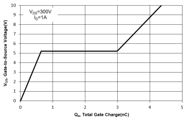
Fig. 11 Gate Charge
