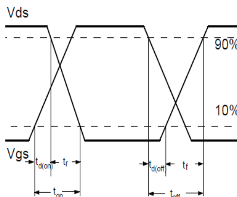
Fig.1-2 Switching Waveform
