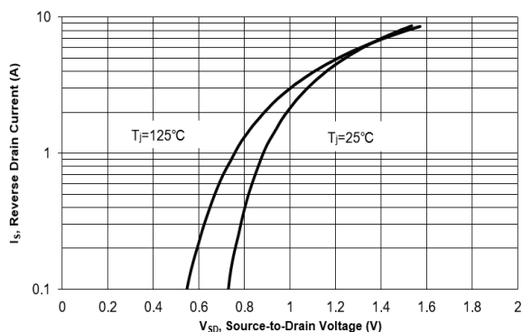
Fig. 6 Typical Body-Diode Forward Characteristics
