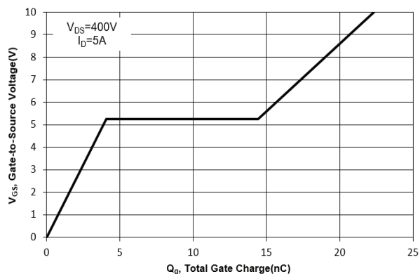
Fig. 11 Gate Charge
