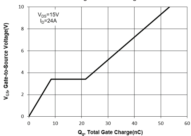
Fig. 11 Gate Charge
