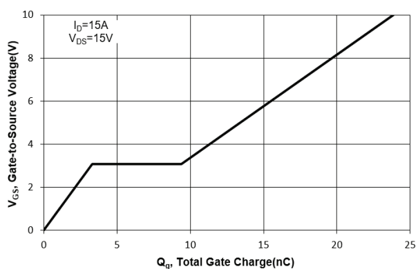
Fig. 11 Gate Charge
