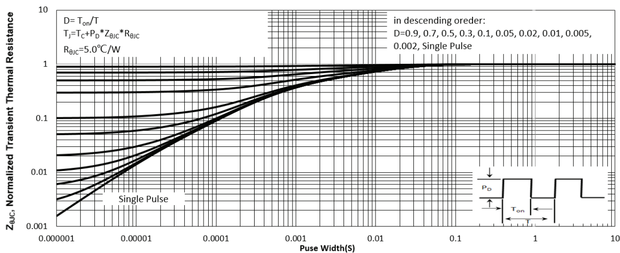
Fig. 13 Normalized Maximum Transient Thermal Impedance( Z_{\theta JC} )
