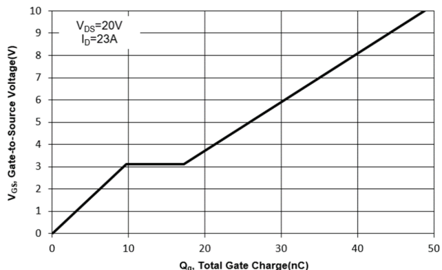
Fig. 11 Gate Charge
