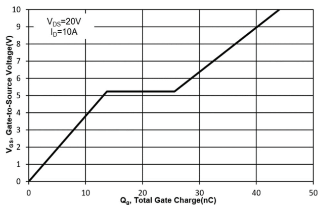
Fig. 11 Gate Charge
