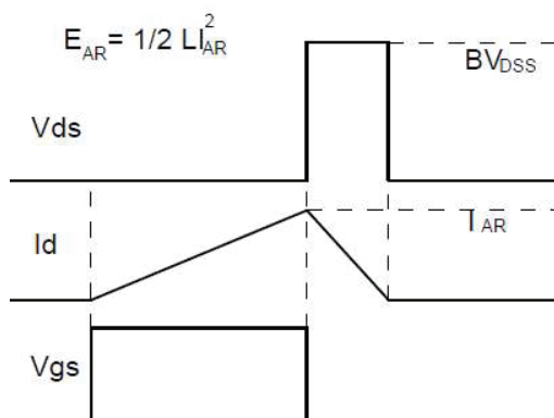
Fig.3-2 Avalanche waveform
