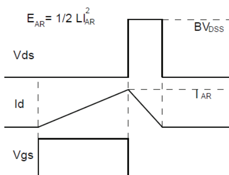
Fig.3-2 Avalanche waveform
