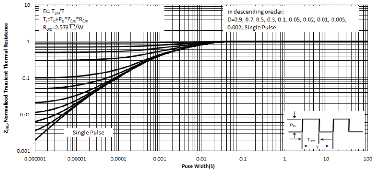
Fig.12 Normalized Maximum Transient Thermal Impedance( Z_{\theta JC} )
