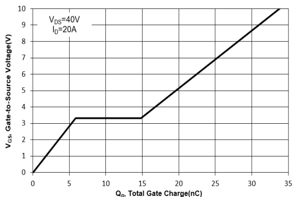
Fig. 11 Gate Charge
