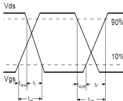
Fig.1-2 Switching Waveform
