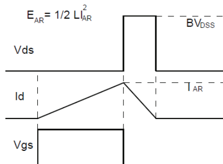
Fig.3-2 Avalanche waveform
