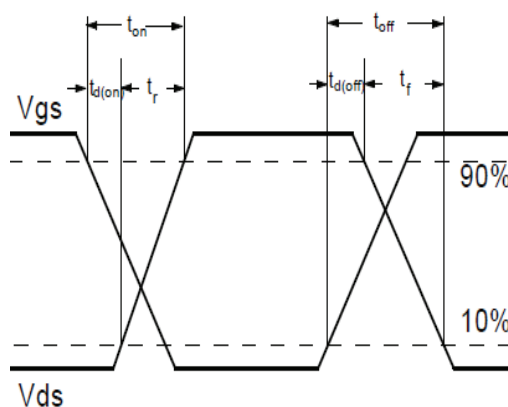
Fig.1-2 Switching Waveform
