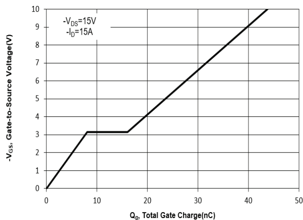
Fig. 11 Gate Charge
