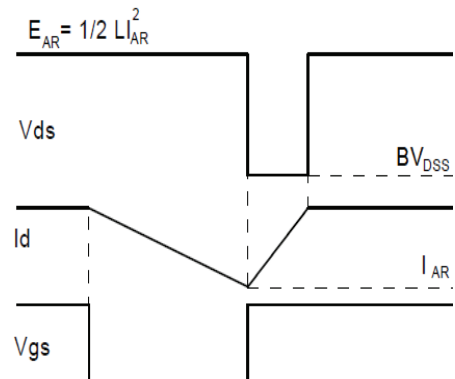
Fig.3-2 Avalanche waveform
