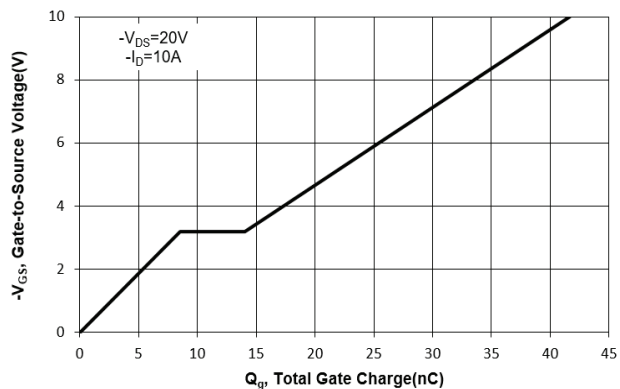
Fig. 11 Gate Charge
