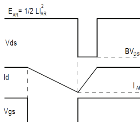
Fig.3-2 Avalanche waveform
