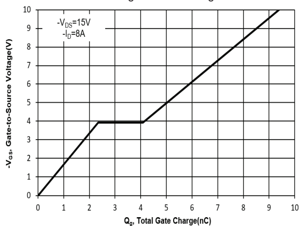
Fig. 11 Gate Charge
