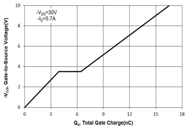
Fig. 11 Gate Charge
