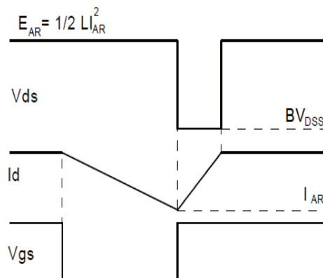
Fig.3-2 Avalanche waveform
