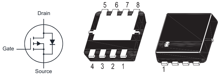
1. Source 2. Source 3. Source 4. Gate 5. Drain 6. Drain 7. Drain 8. Drain DFN3030 Plastic Package
