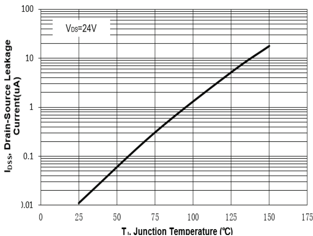
Fig. 11 Drain-Source Leakage Current vs. T_J
