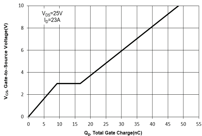
Fig. 11 Gate Charge
