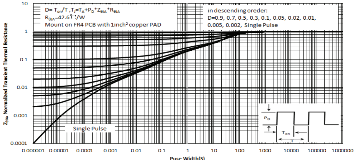
Fig.13 Normalized Maximum Transient Thermal Impedance( Z_{\theta JA} )
