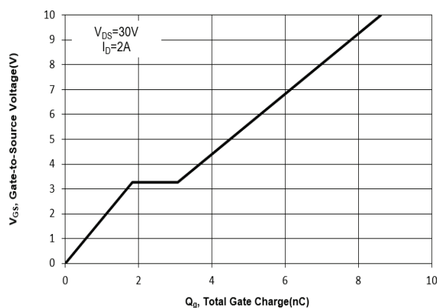
Fig. 11 Gate Charge
