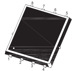
1.Source 2.Source 3.Source 4.Gate 5.Drain 6.Drain 7.Drain 8.Drain DFN5060 Plastic Package
