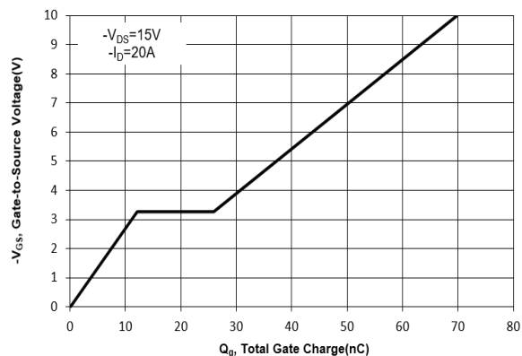
Fig. 11 Gate Charge
