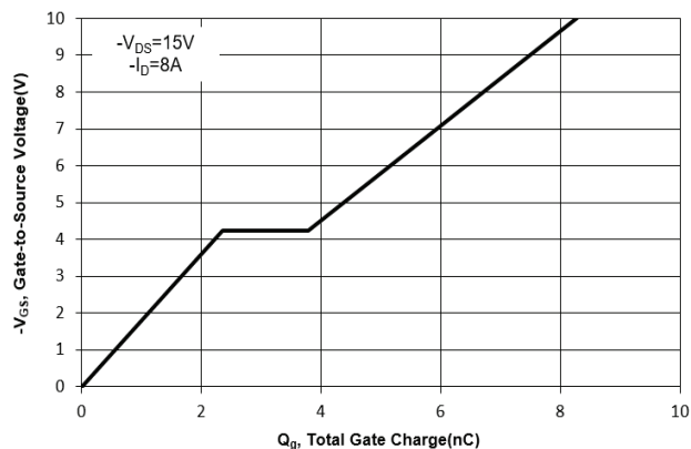
Fig. 11 Gate Charge
