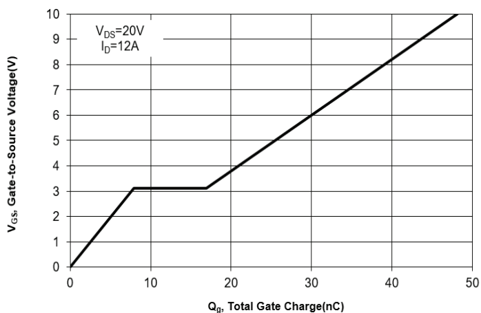
Fig. 11 Gate Charge
