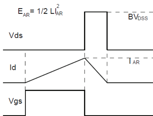
Fig.3-2 Avalanche waveform
