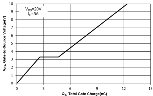
Fig. 11 Gate Charge
