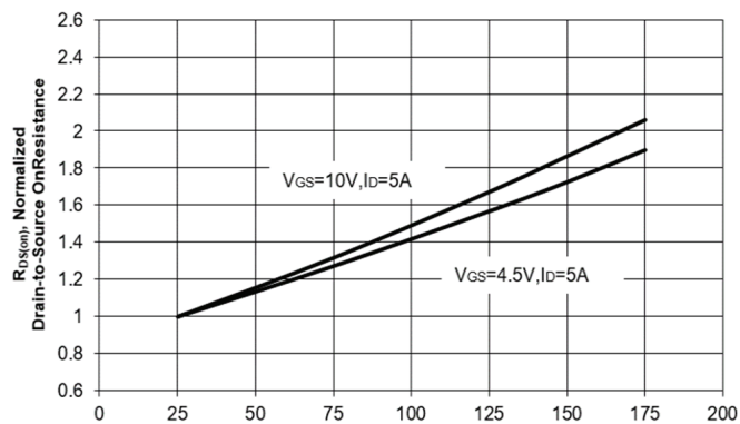
Fig. 5 On-Resistance vs. T_j
