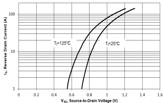
Fig. 6 Typical Forward Body-Diode Characteristics
