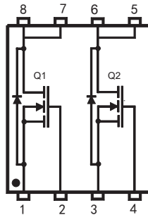
Q1:1.Source 2.Gate 7.Drain 8.Drain Q2:3.Source 4.Gate 5.Drain 6.Drain DFN5060 Plastic Package
