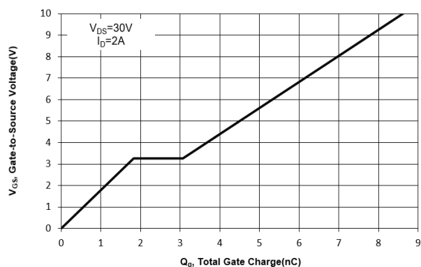
Fig. 11 Gate Charge
