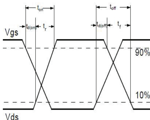
Fig.1-2 Switching Waveform
