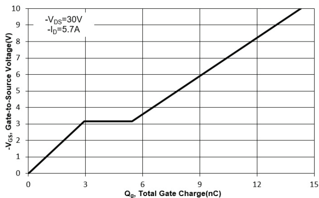
Fig. 11 Gate Charge
