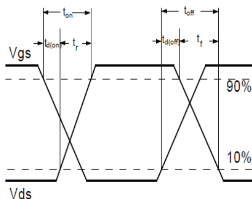
Fig.1-2 Switching Waveform
