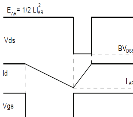
Fig.3-2 Avalanche waveform
