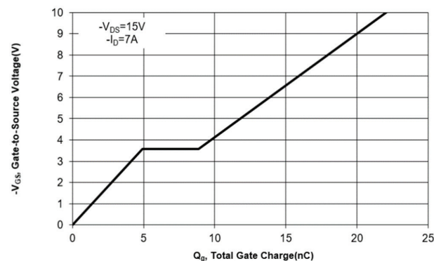
Fig. 11 Gate Charge
