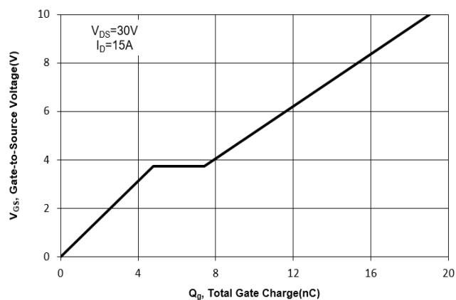
Fig. 11 Gate Charge
