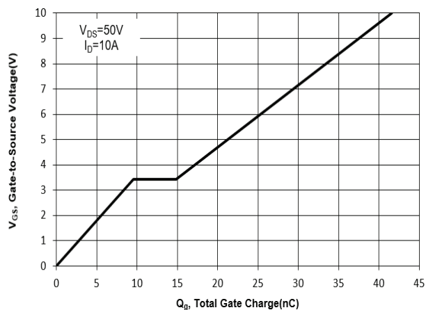
Fig. 11 Gate Charge
