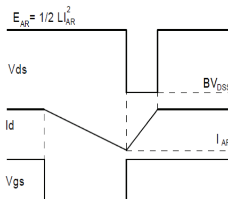
Fig.3-2 Avalanche waveform
