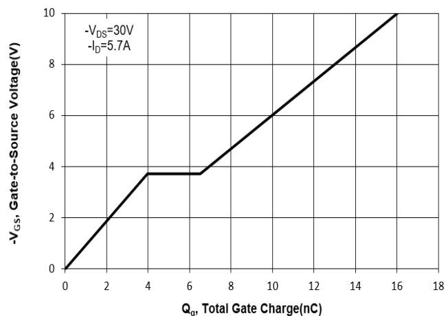
Fig. 11 Gate Charge
