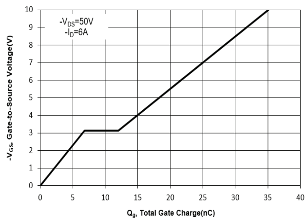
Fig. 11 Gate Charge
