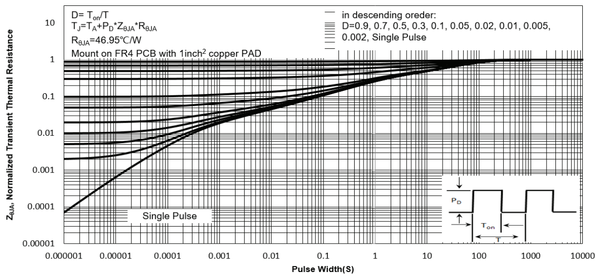
Fig. 13 Normalized Maximum Transient Thermal Impedance( Z_{\theta JA} )
