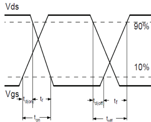
Fig.1-2 Switching Waveform
