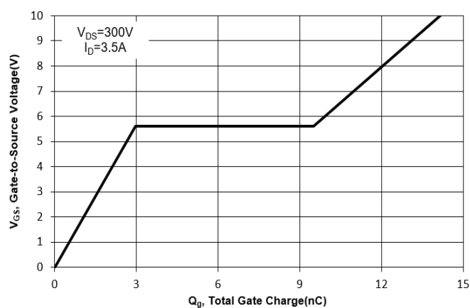
Fig. 11 Gate Charge
