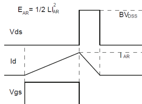
Fig.3-2 Avalanche waveform
