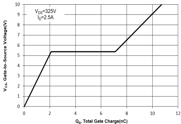
Fig. 11 Gate Charge
